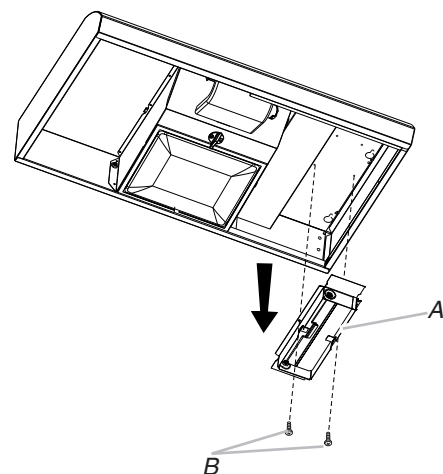
A. 3\frac{1}{4}" \times 10" (8.3 x 25.4 cm) rectangular vent damper B. Screws
